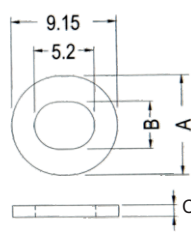
WSR8.65*4.1-1.0(9.15)
