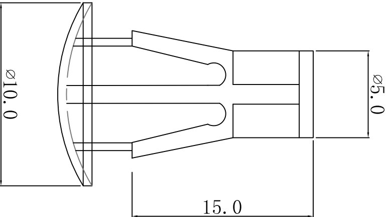
CHASSIS \phi 5.5 THICKNESS 0.8-1.6
